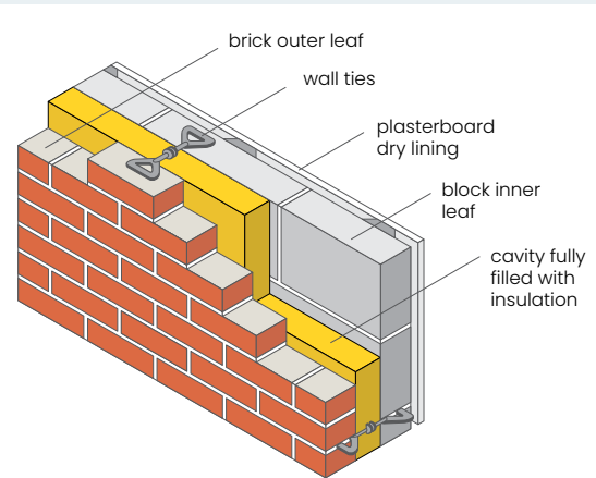
Cavity fully filled with insulation
