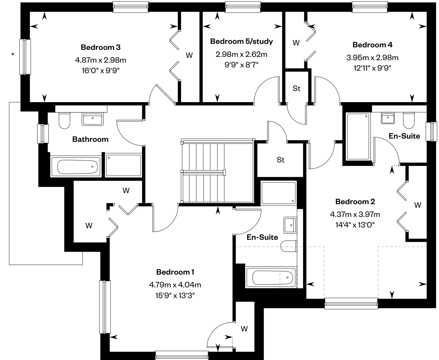
First floor
