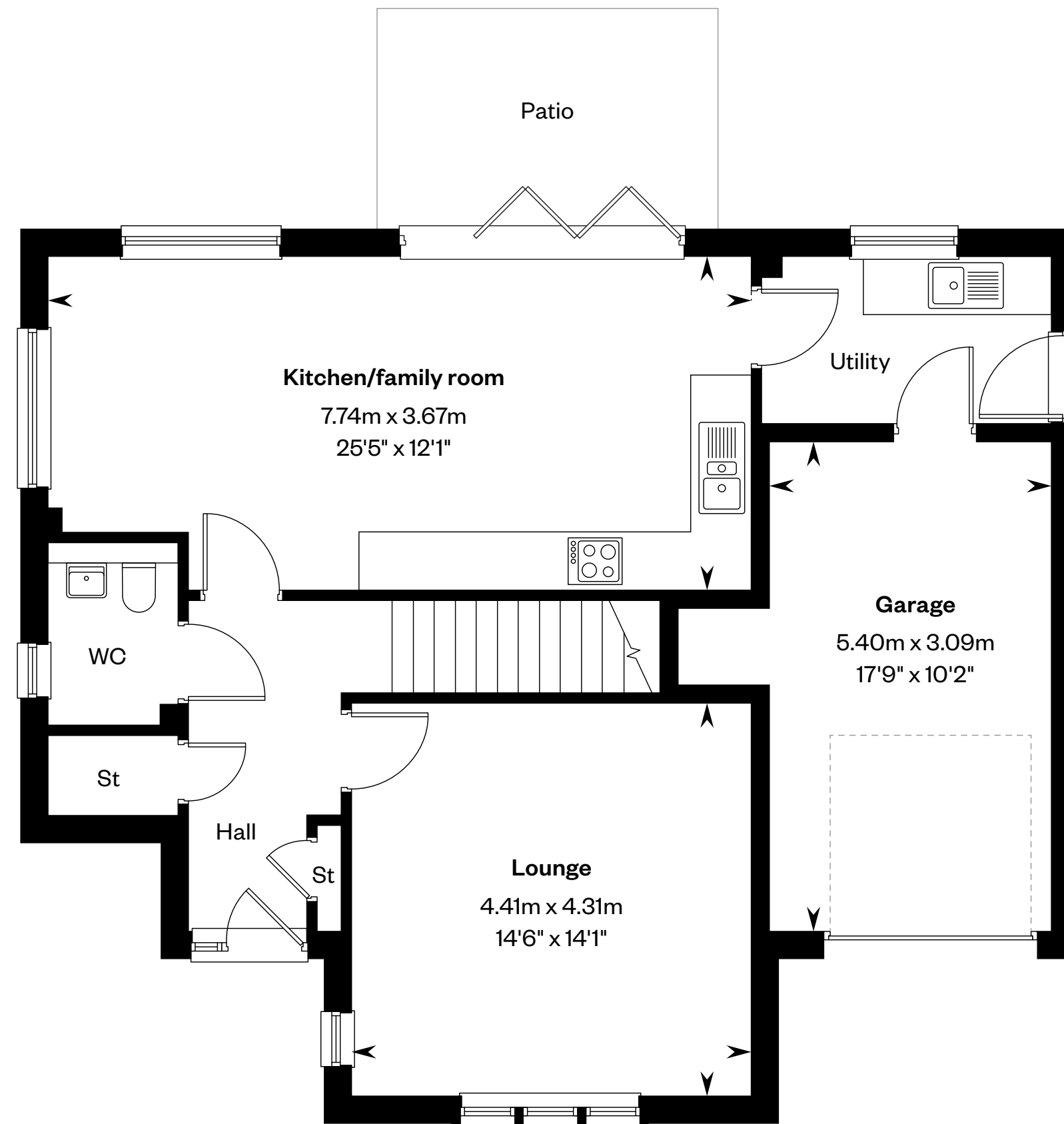
Ground floor
