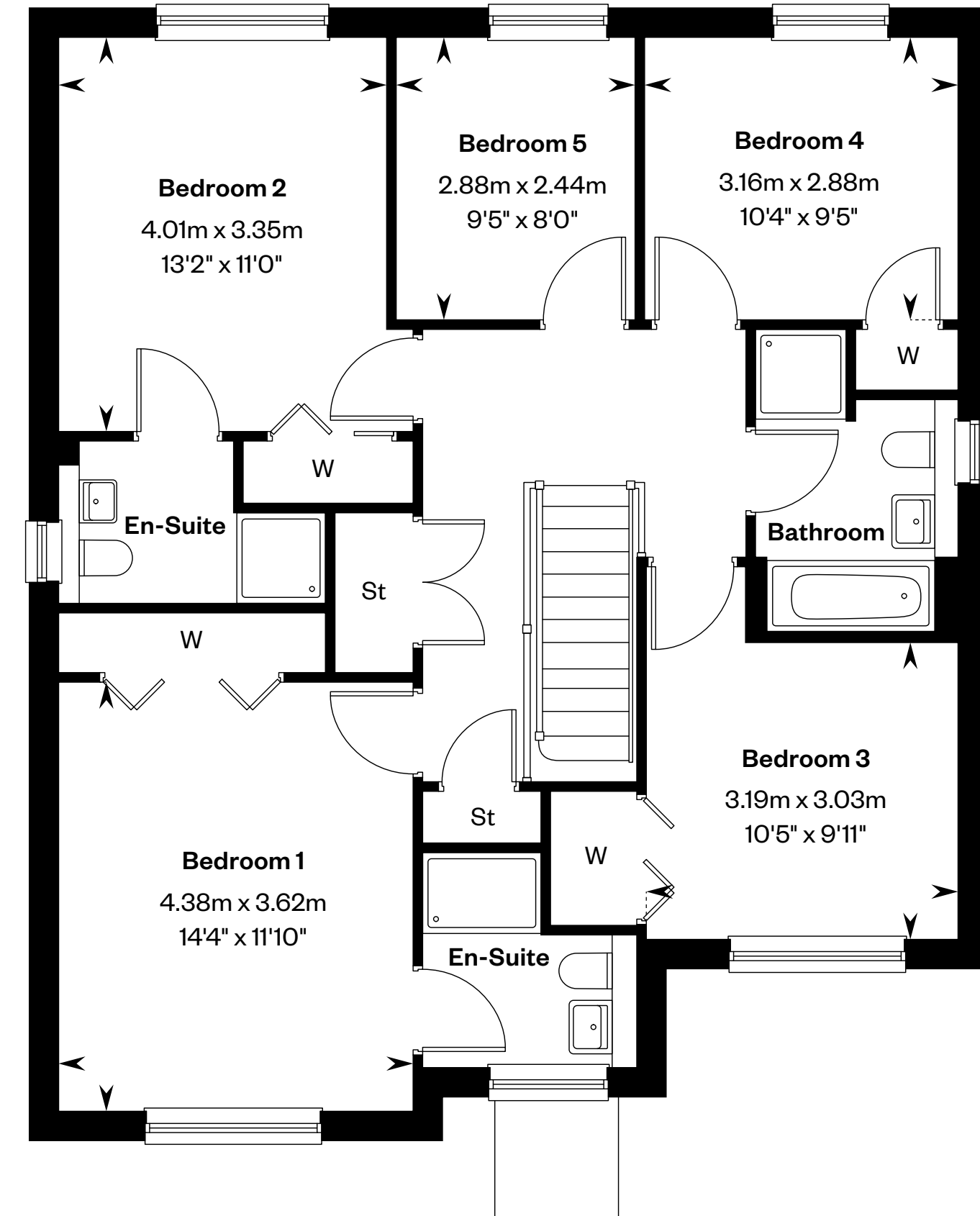
First floor
