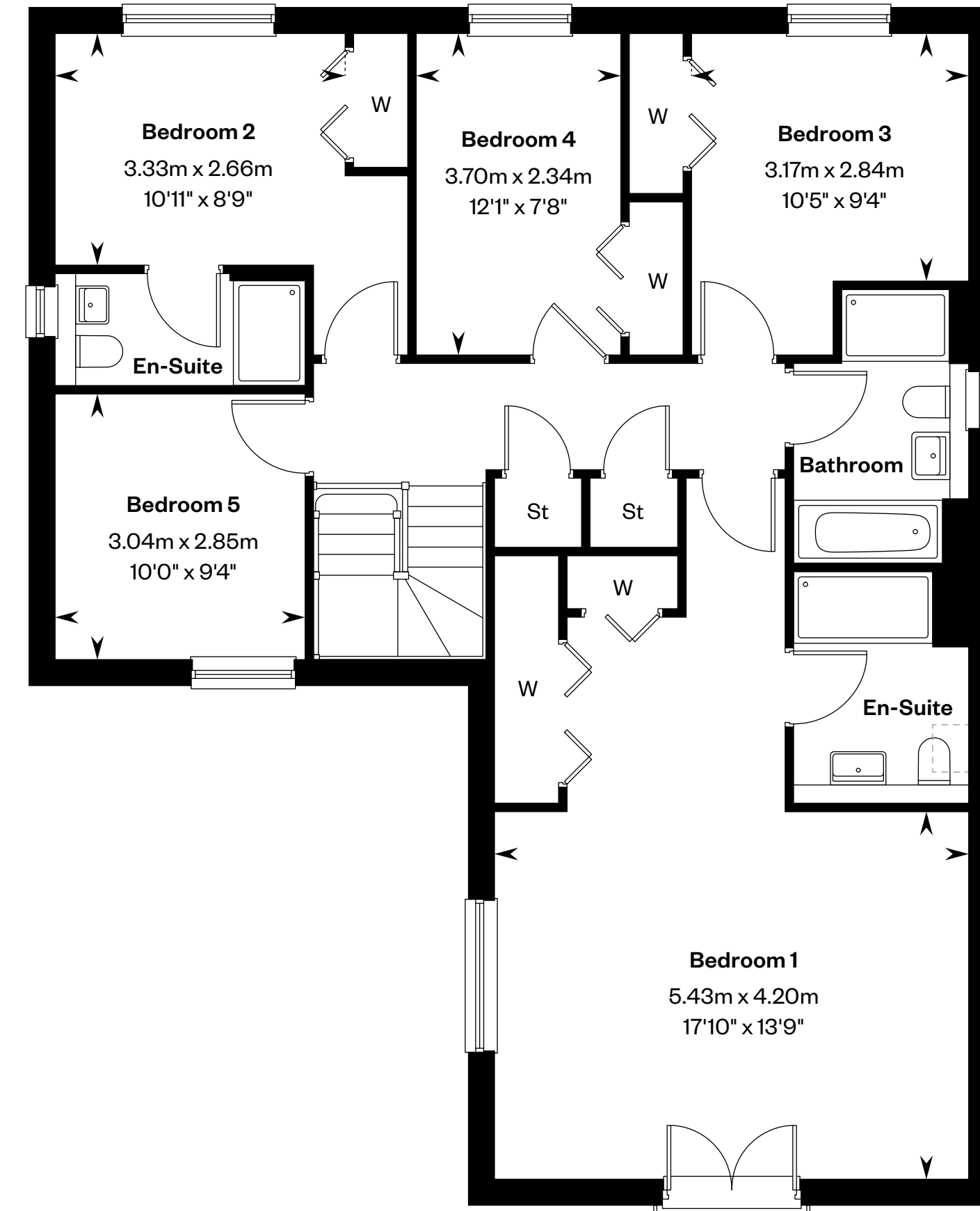
First floor
