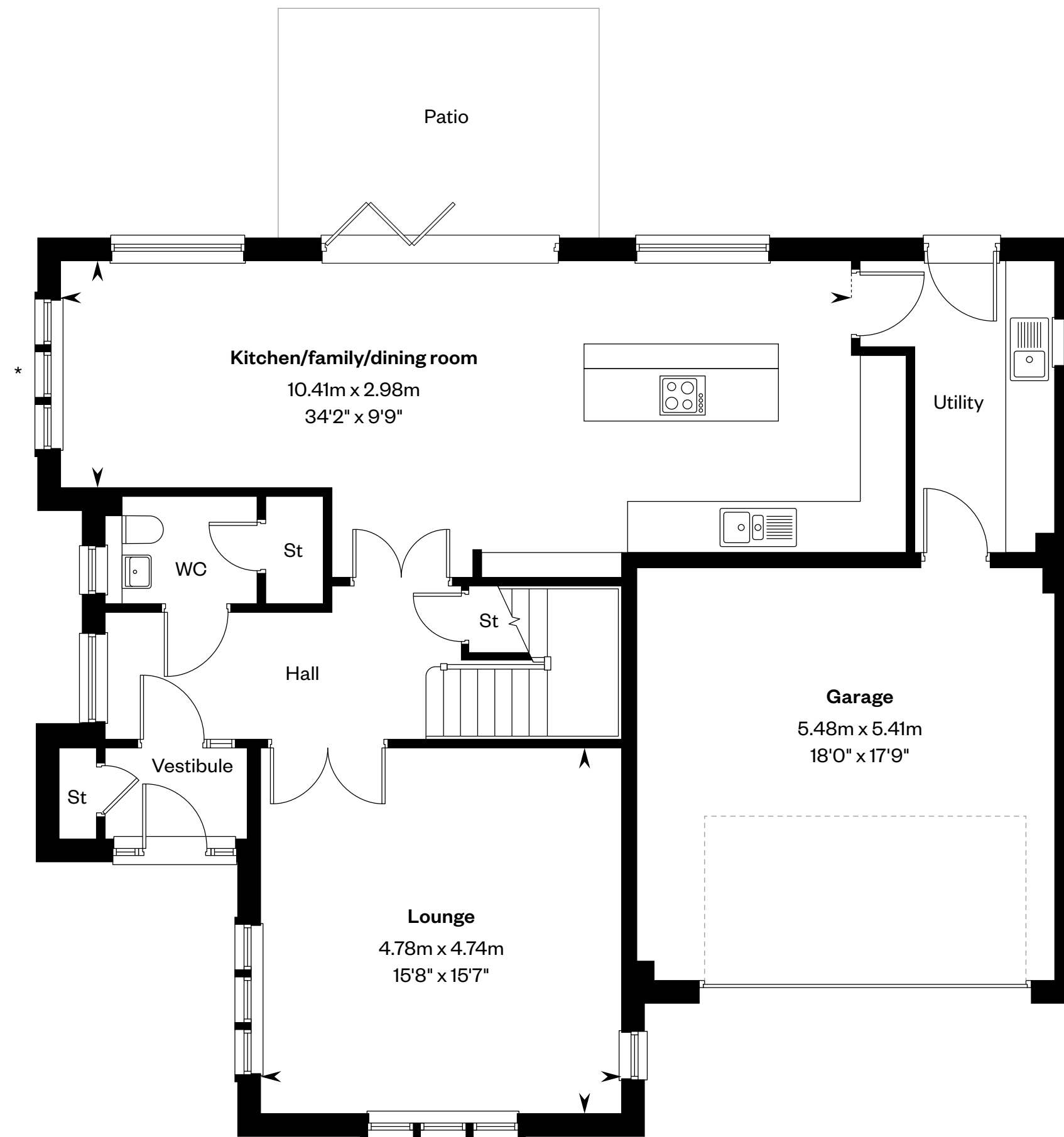
Ground floor
