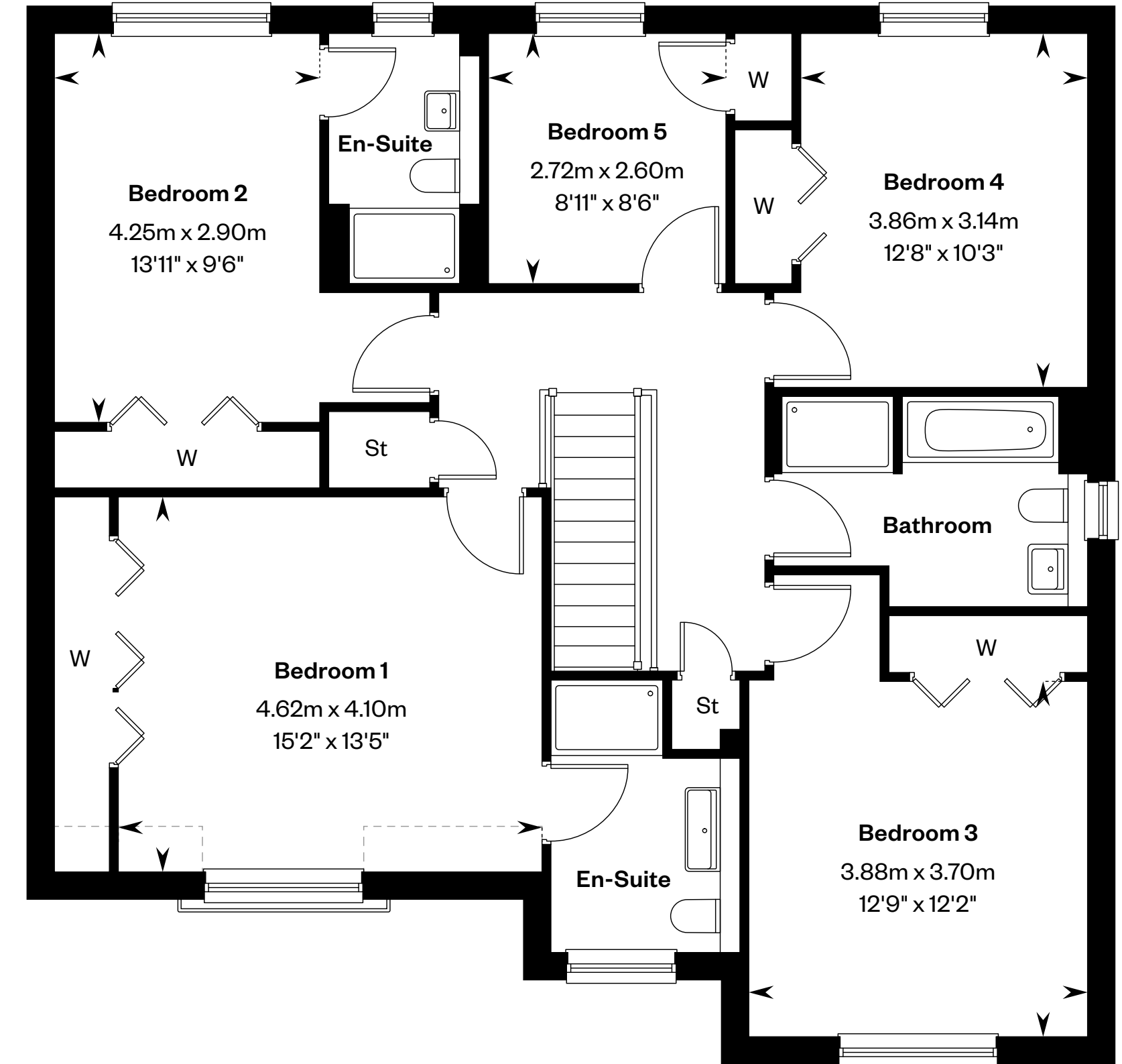
First floor
