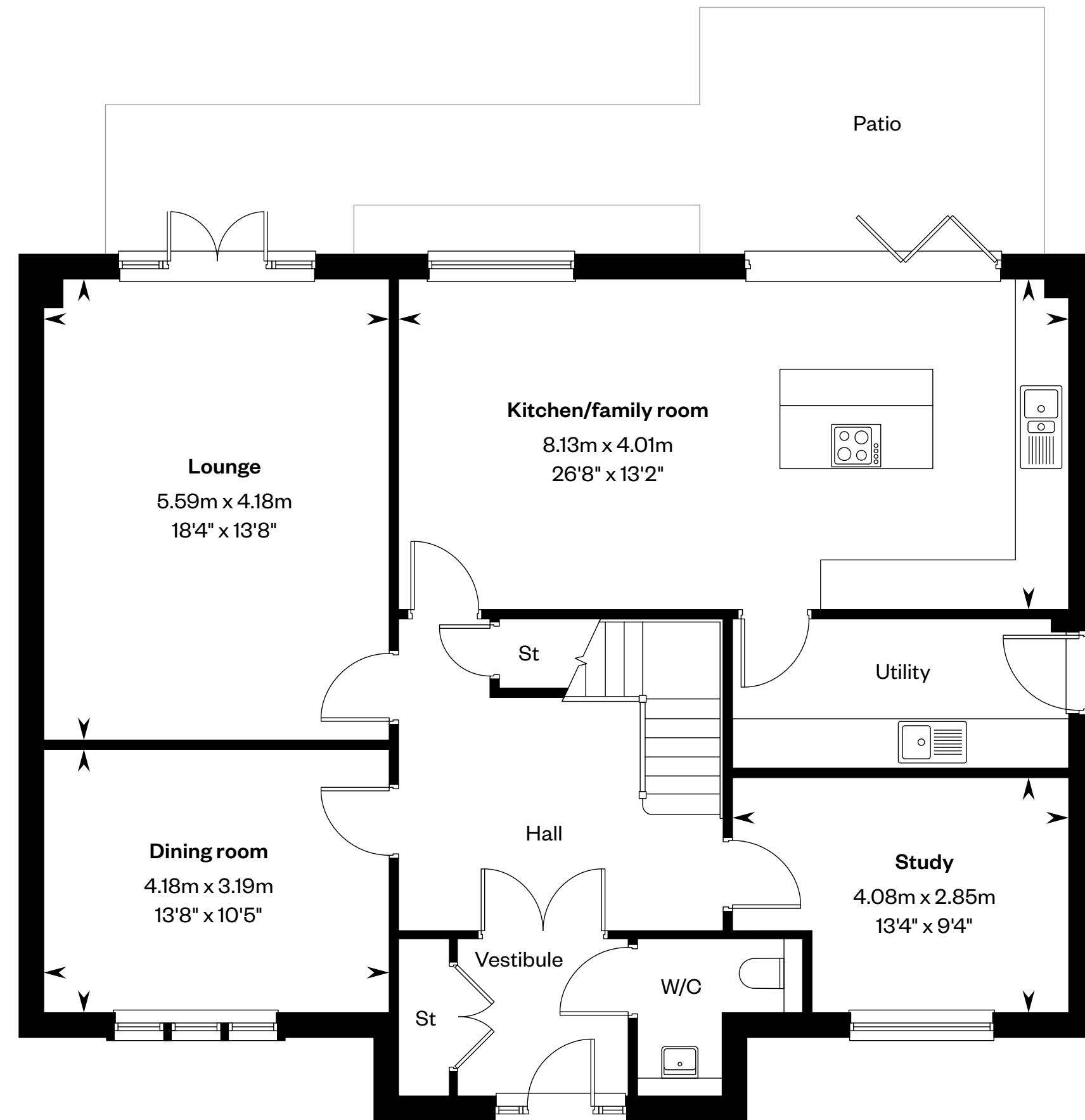
Ground floor
