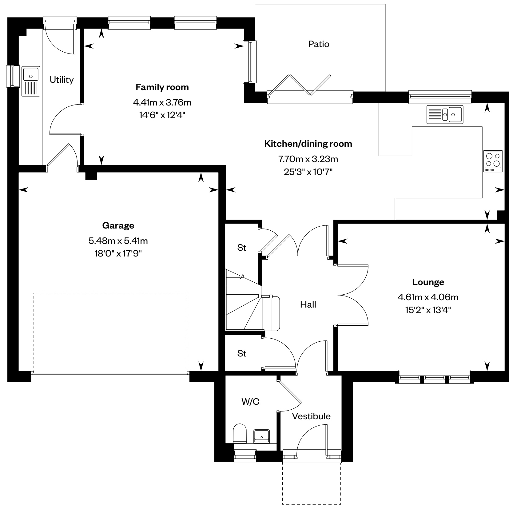
Ground floor
