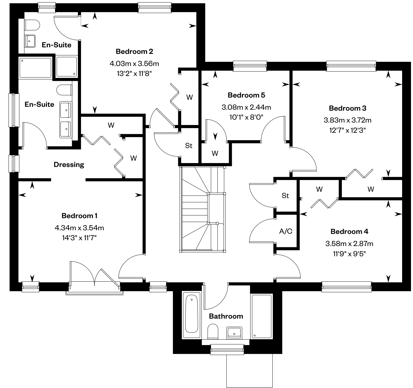
First floor
