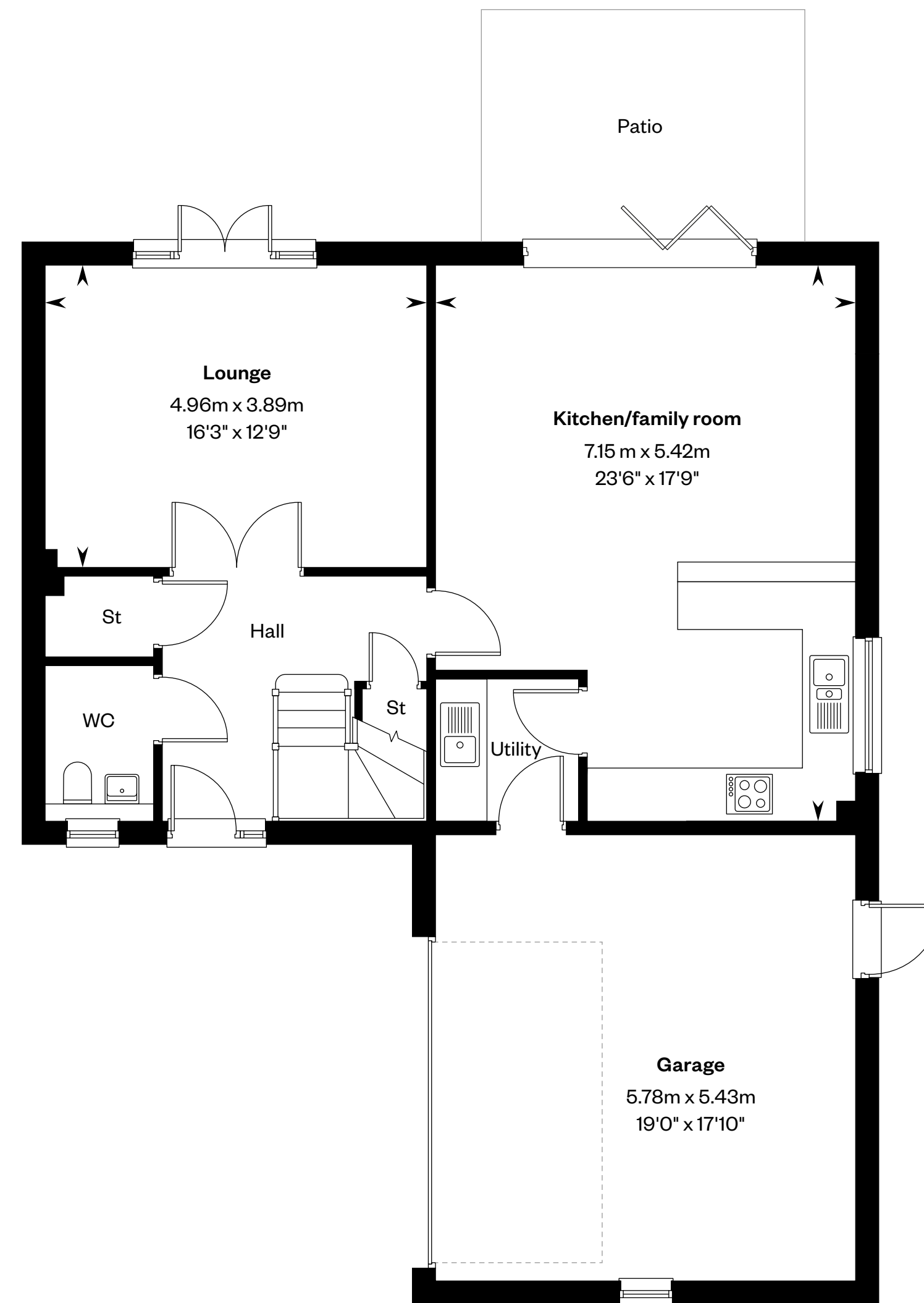
Ground floor
