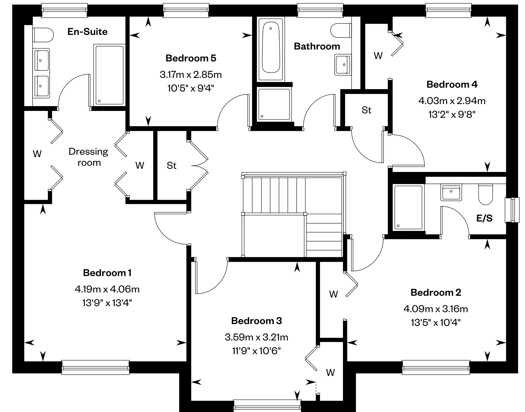
First floor
