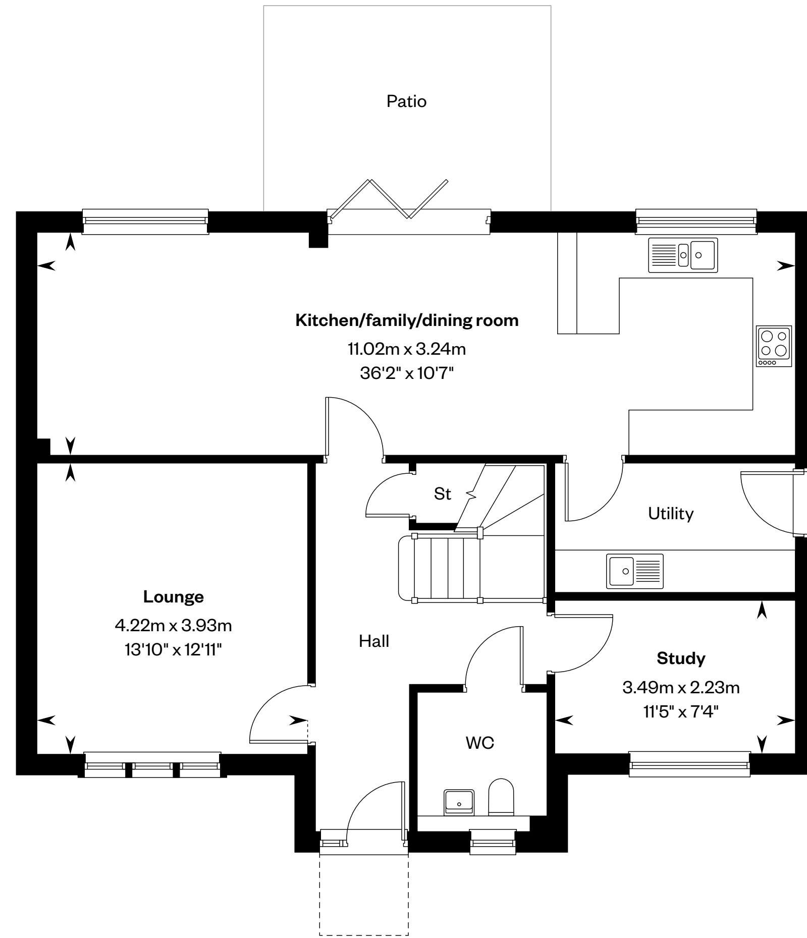
Ground floor
