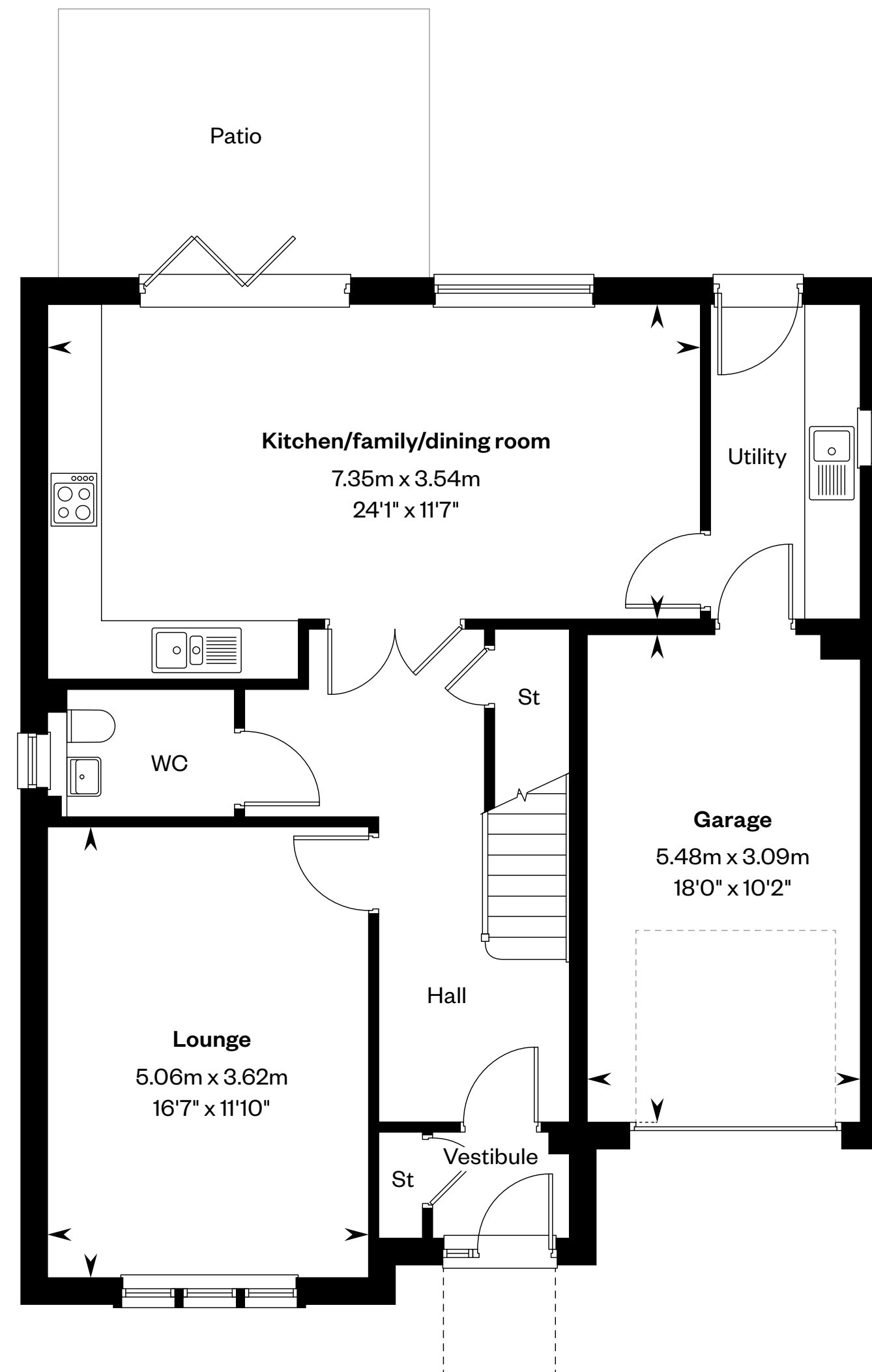
Ground floor
