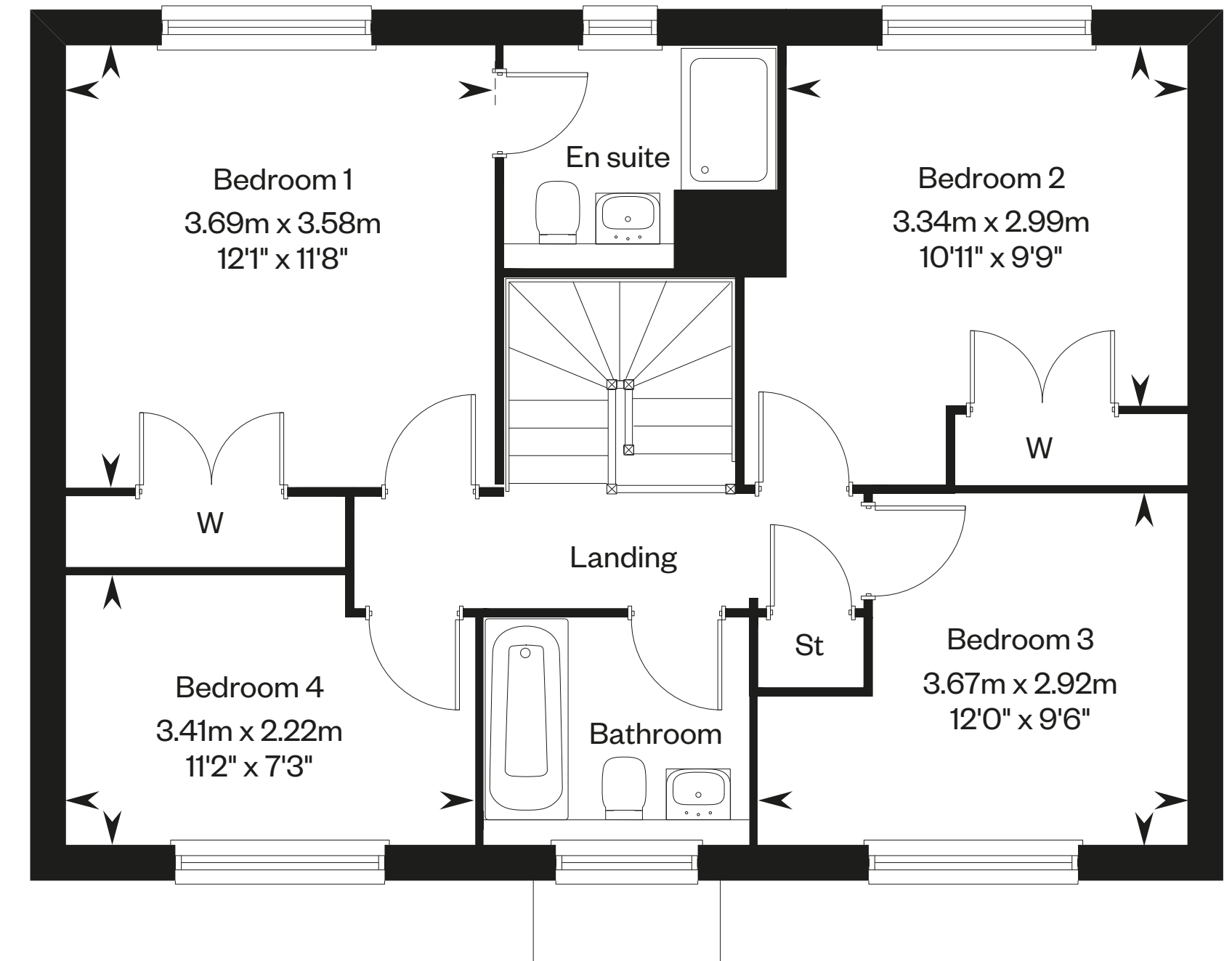
First floor
