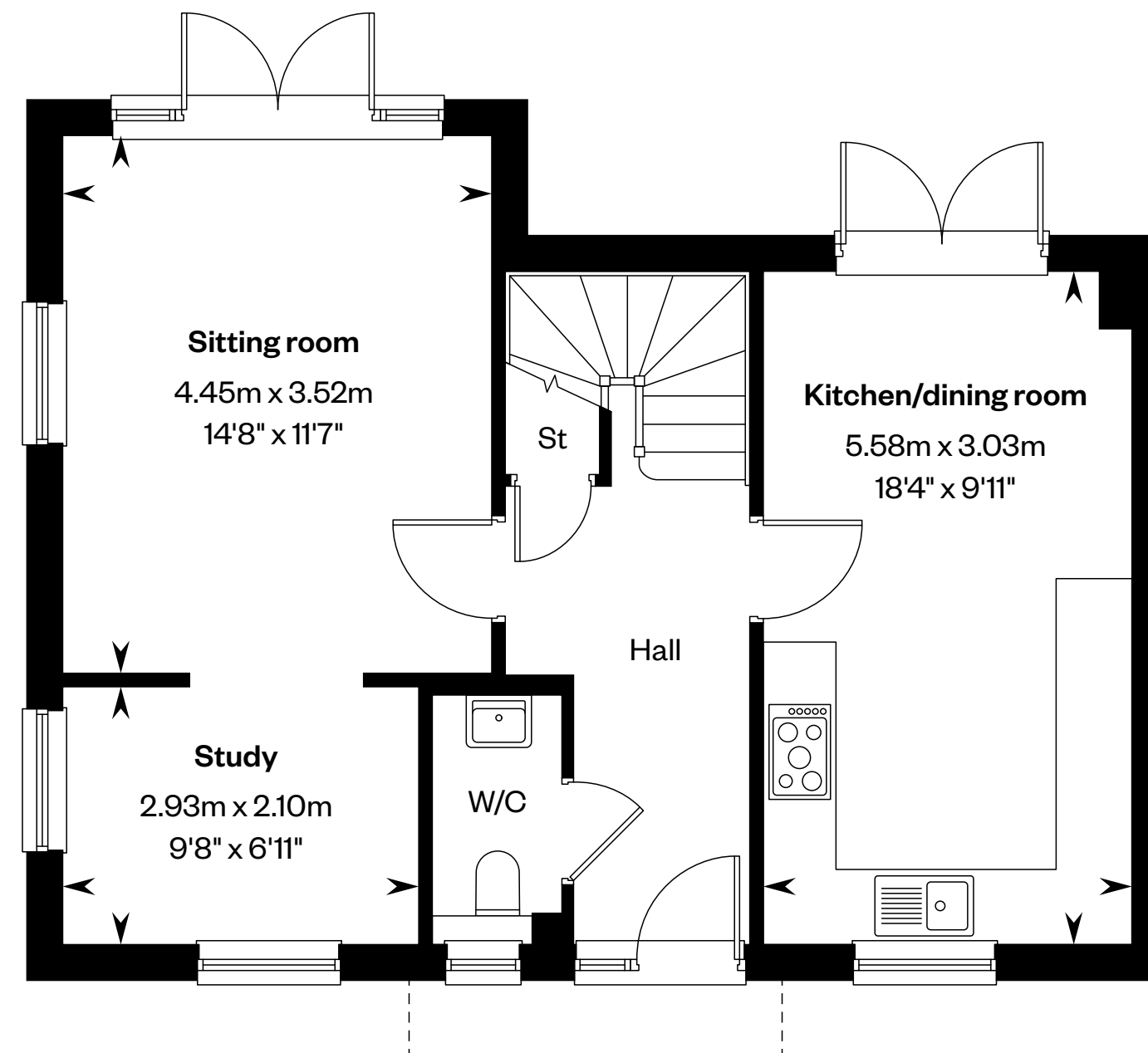
Ground floor
