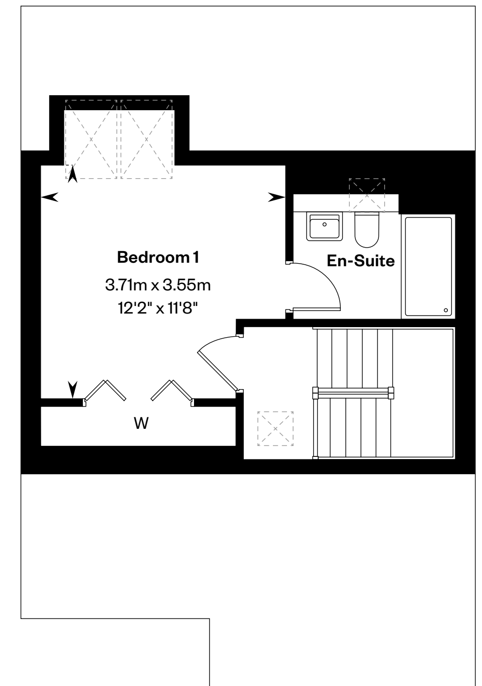
Second floor
