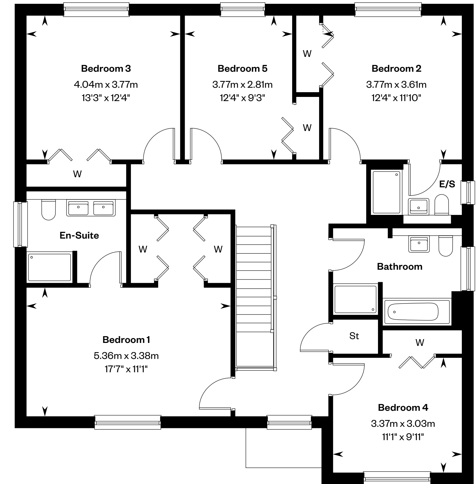
First floor
