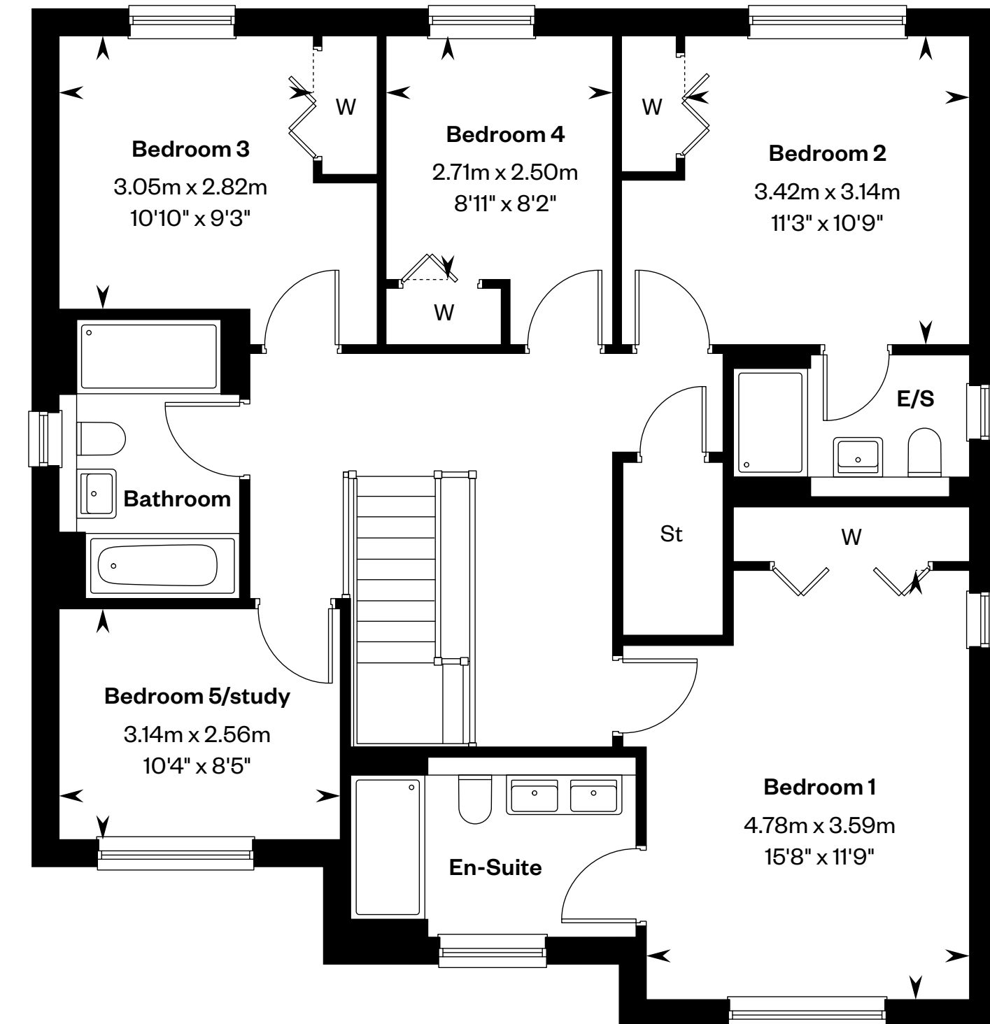
First floor
