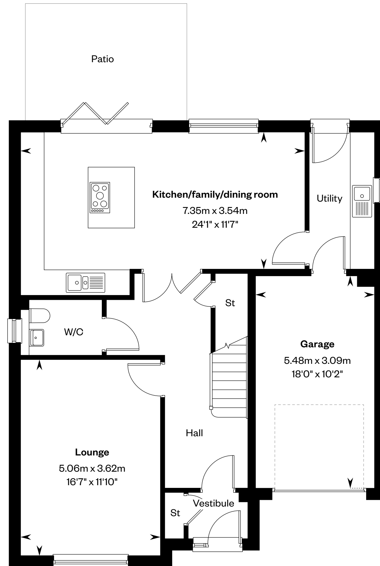
Ground floor
