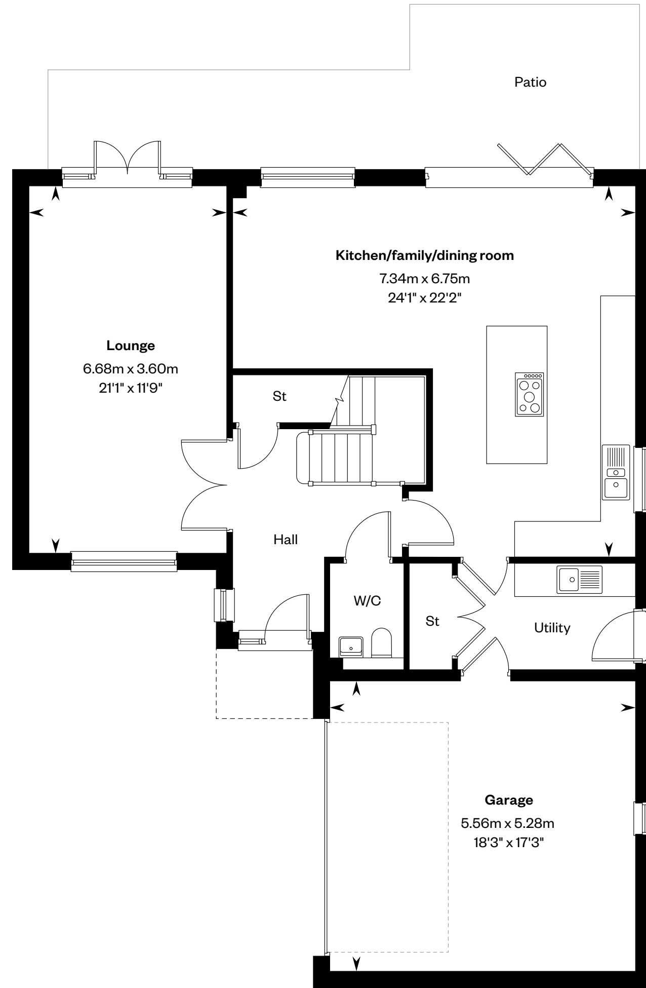
Ground floor
