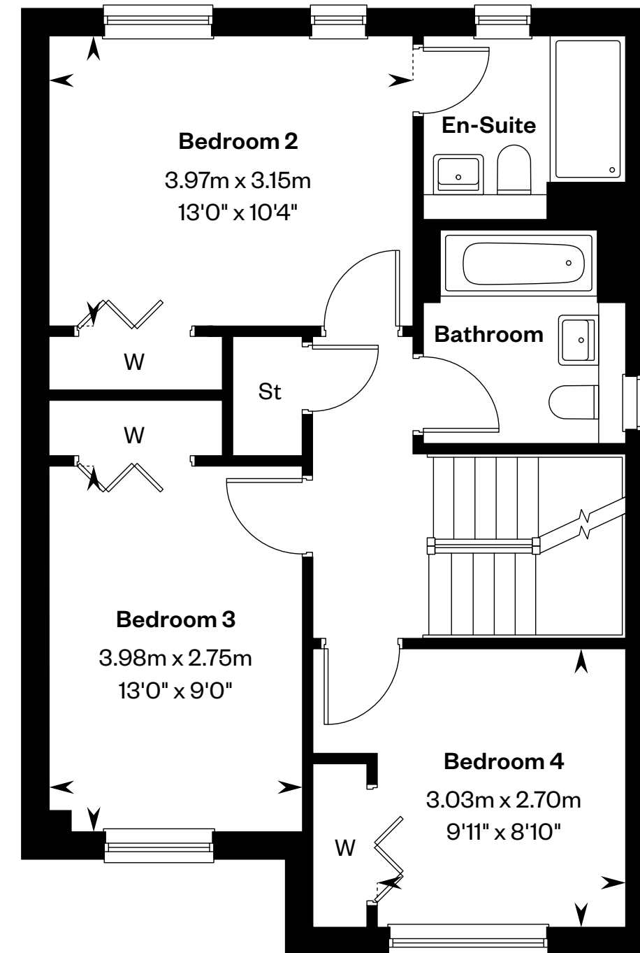
First floor
